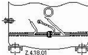
Figure 13: Crankcase heater location, models ZR94K* to ZR380K* & ZP103K* to ZP485K*
